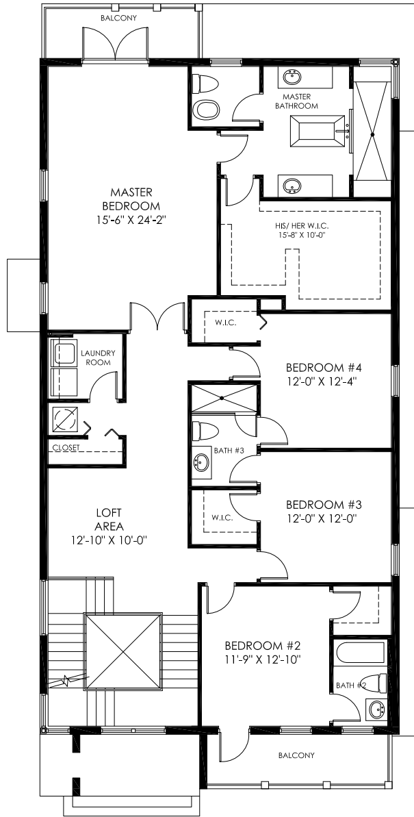
UNIT TYPE "C-ALT" SECOND FLOOR
