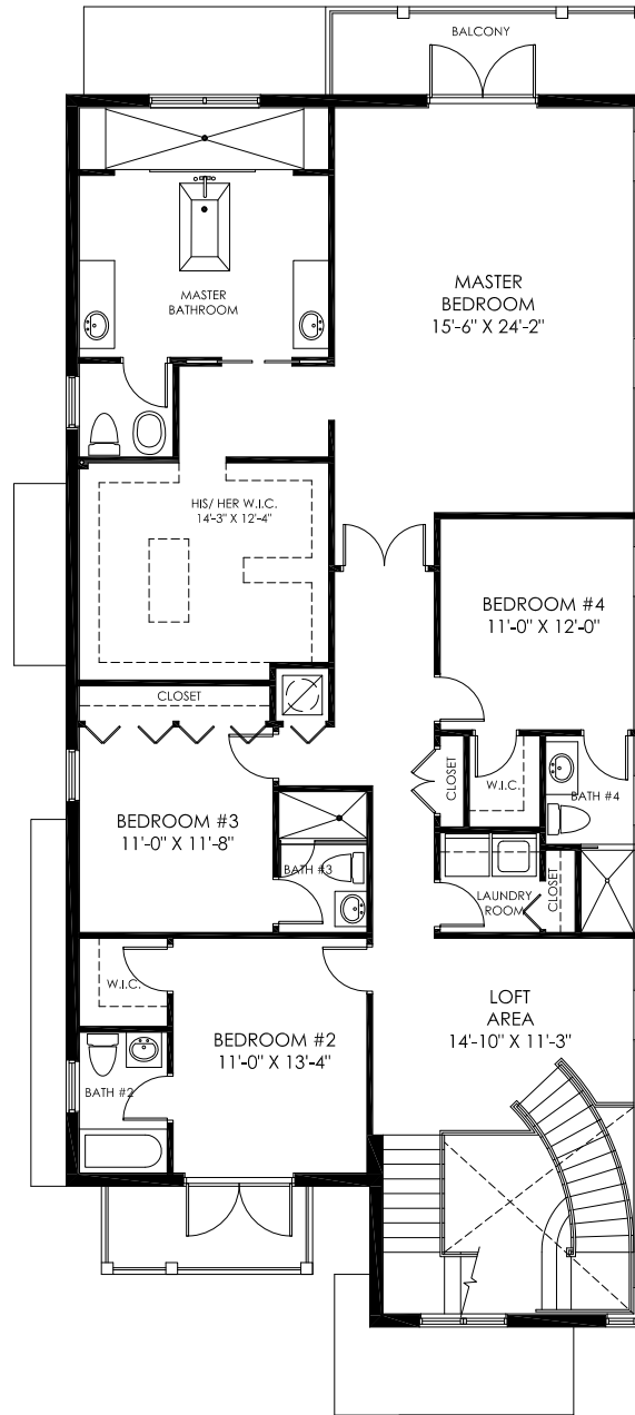
UNIT TYPE "D-ALT" SECOND FLOOR
