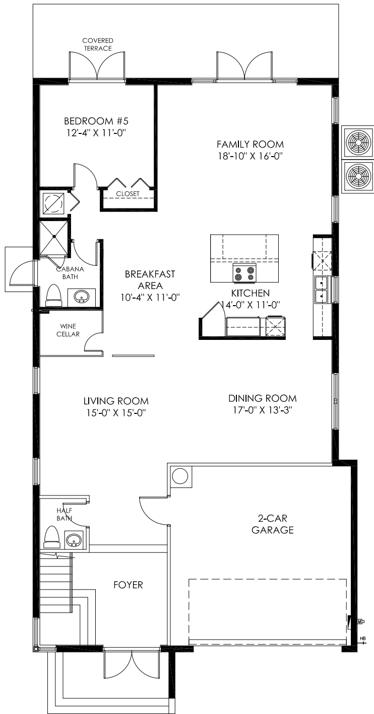
UNIT TYPE "C" GROUND FLOOR
