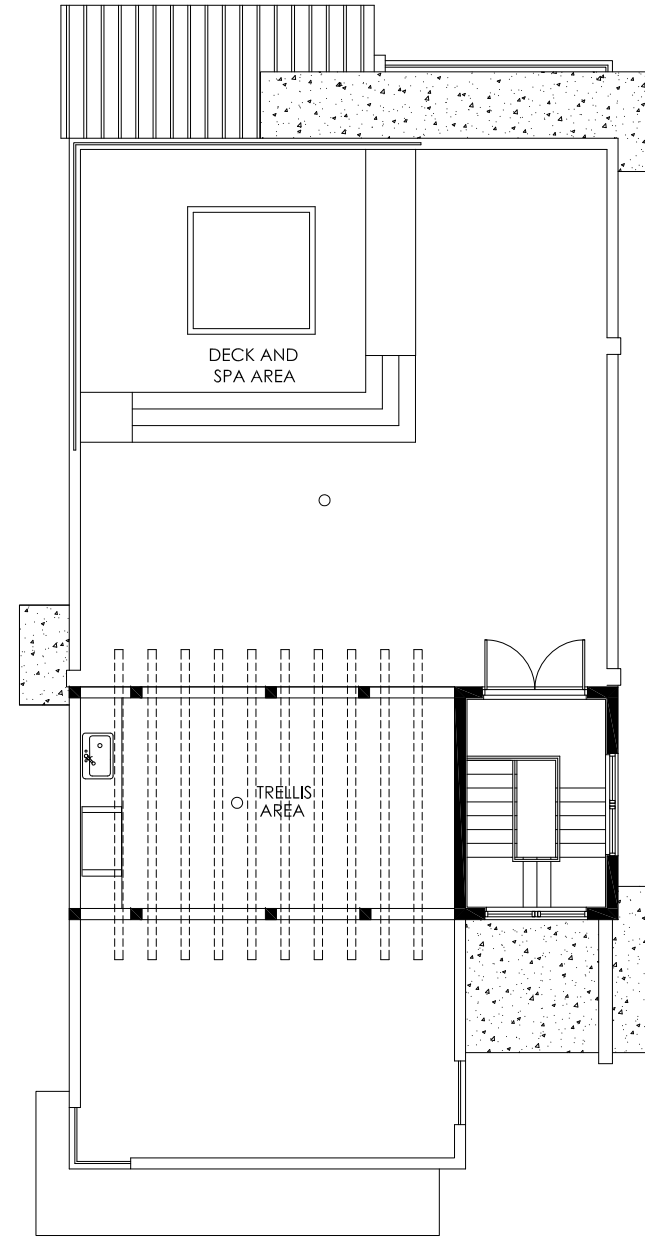
UNIT TYPE "A-ALT" ROOF DECK
