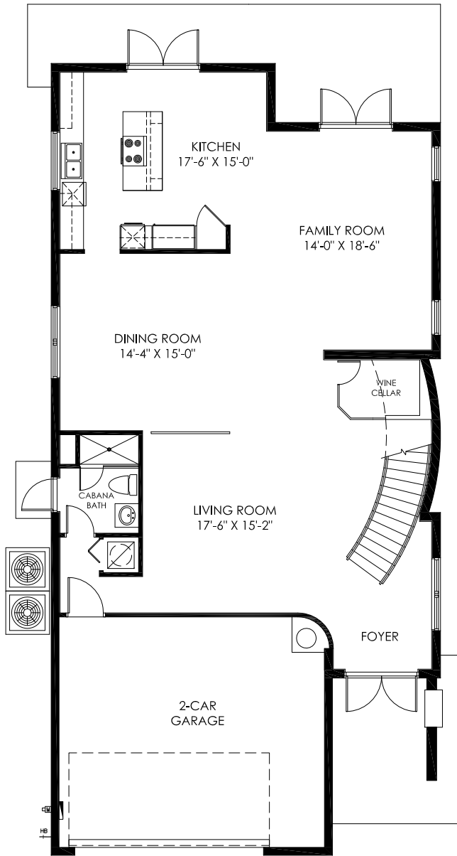
UNIT TYPE "A-ALT" GROUND FLOOR
